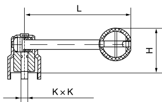
圆压盖拉杆手柄 | 2040002 Circular Pulling handle
