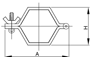
六角型管支架 Hexagon pipe holder 3180015
