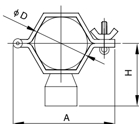
六角型管支架带柄 Hexagon pipe holder with handle 3181018
