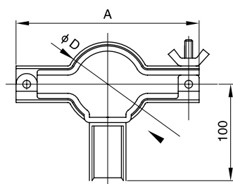
六角型管支架带柄 Hexagon pipe holder with handle 3181017
