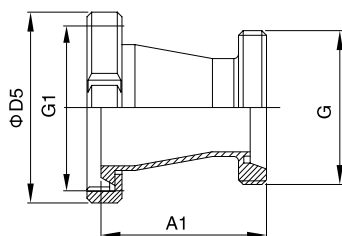
(单螺纹单螺母 Threaded/nut)
