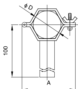
六角型管支架带柄 Hexagon pipe holder with handle 3181018
