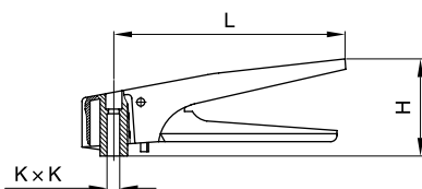
多位不锈钢手柄 | 2040004 Multi-position stainless steel handle
